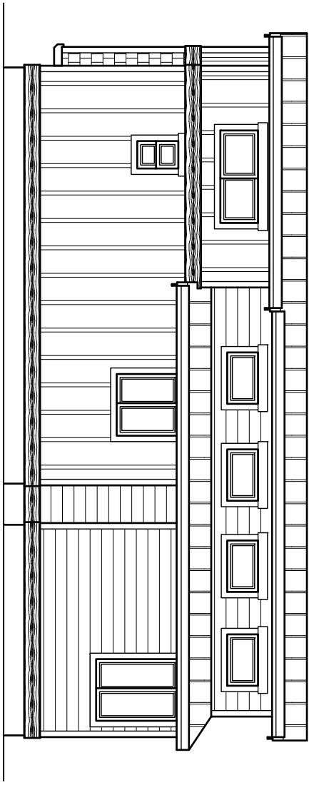
SIDE ELEVATION
