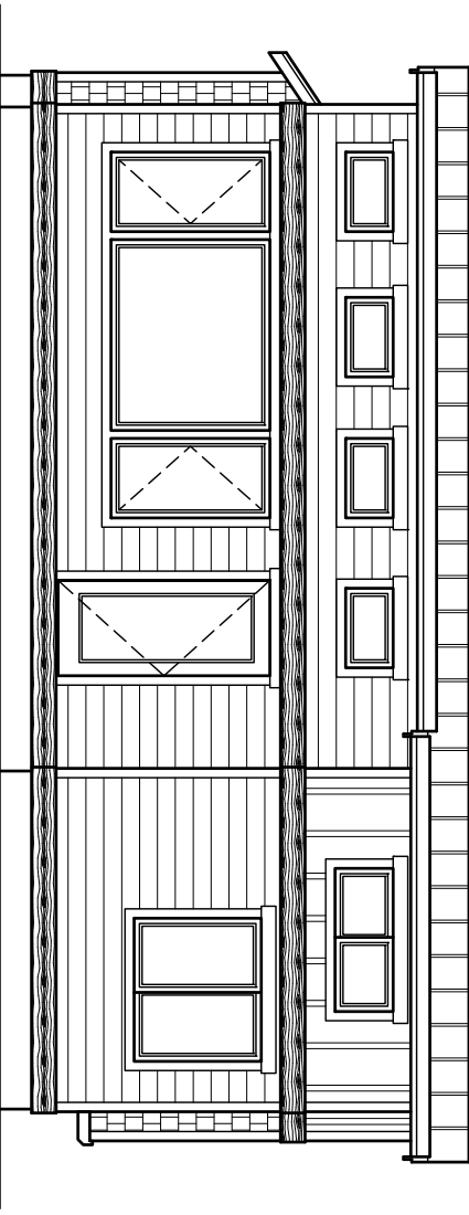
SIDE ELEVATION
